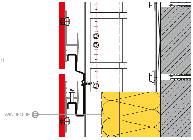
HORIZONTALFUGE A110
