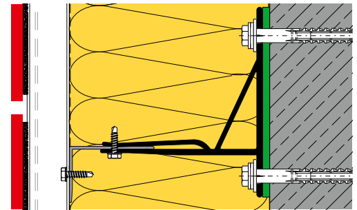
HORIZONTALFUGE A110
