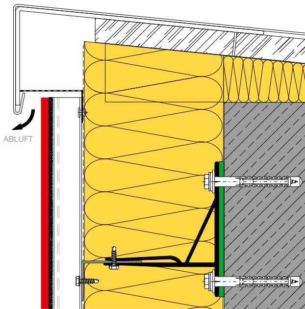
ATTIKA A109
