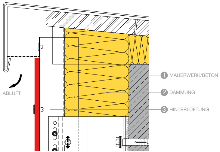
ATTIKA A109
