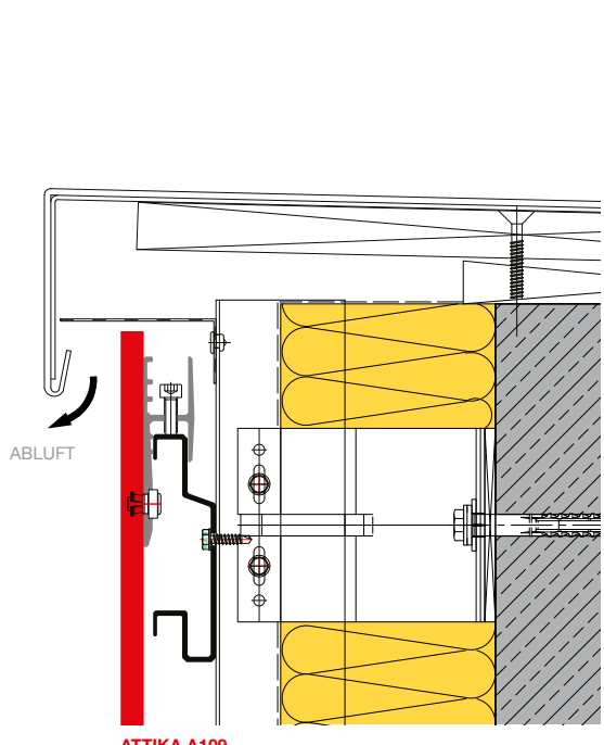
ATTIKA A109
