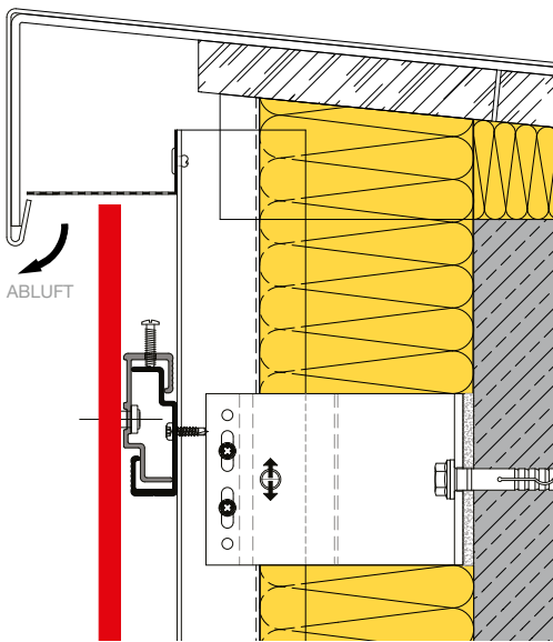
ATTIKA A109
