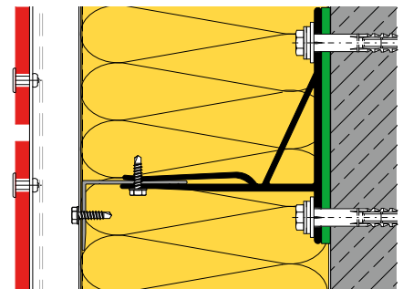
HORIZONTALFUGE A110
