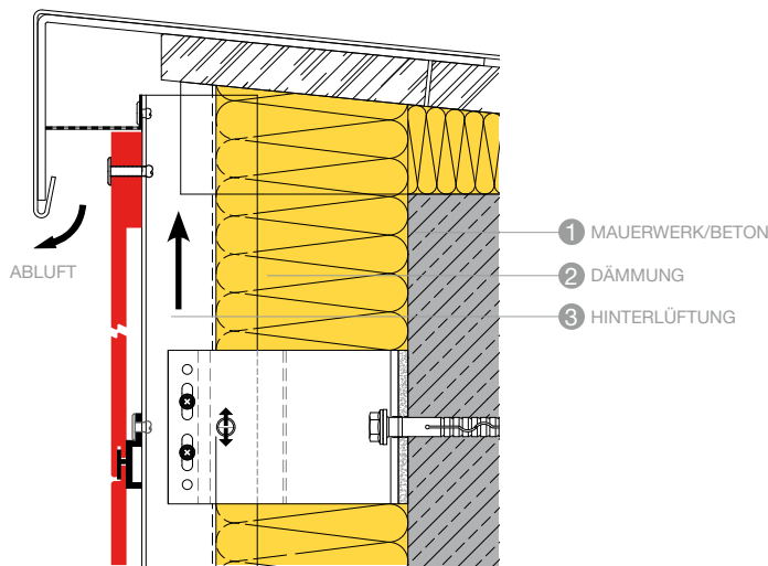
ATTIKA A109
